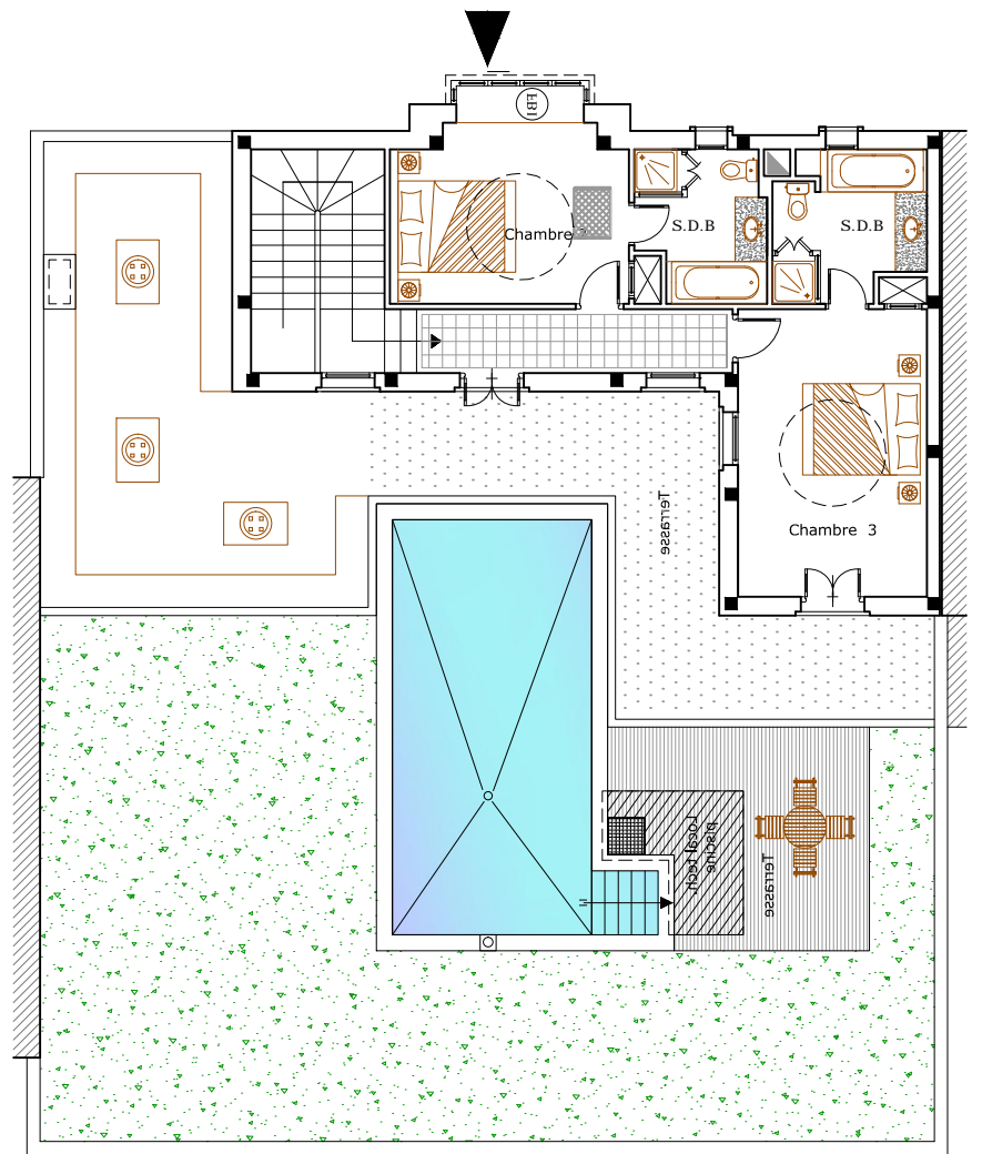
PLAN R+1
